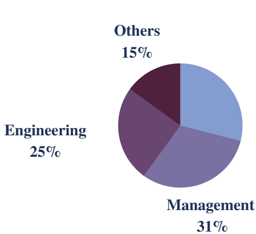
SYMMS Batch Profile
