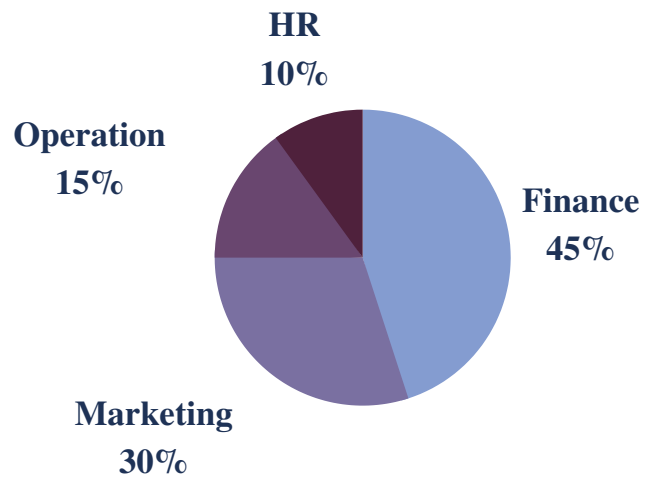
SYMMS Batch Distribution
